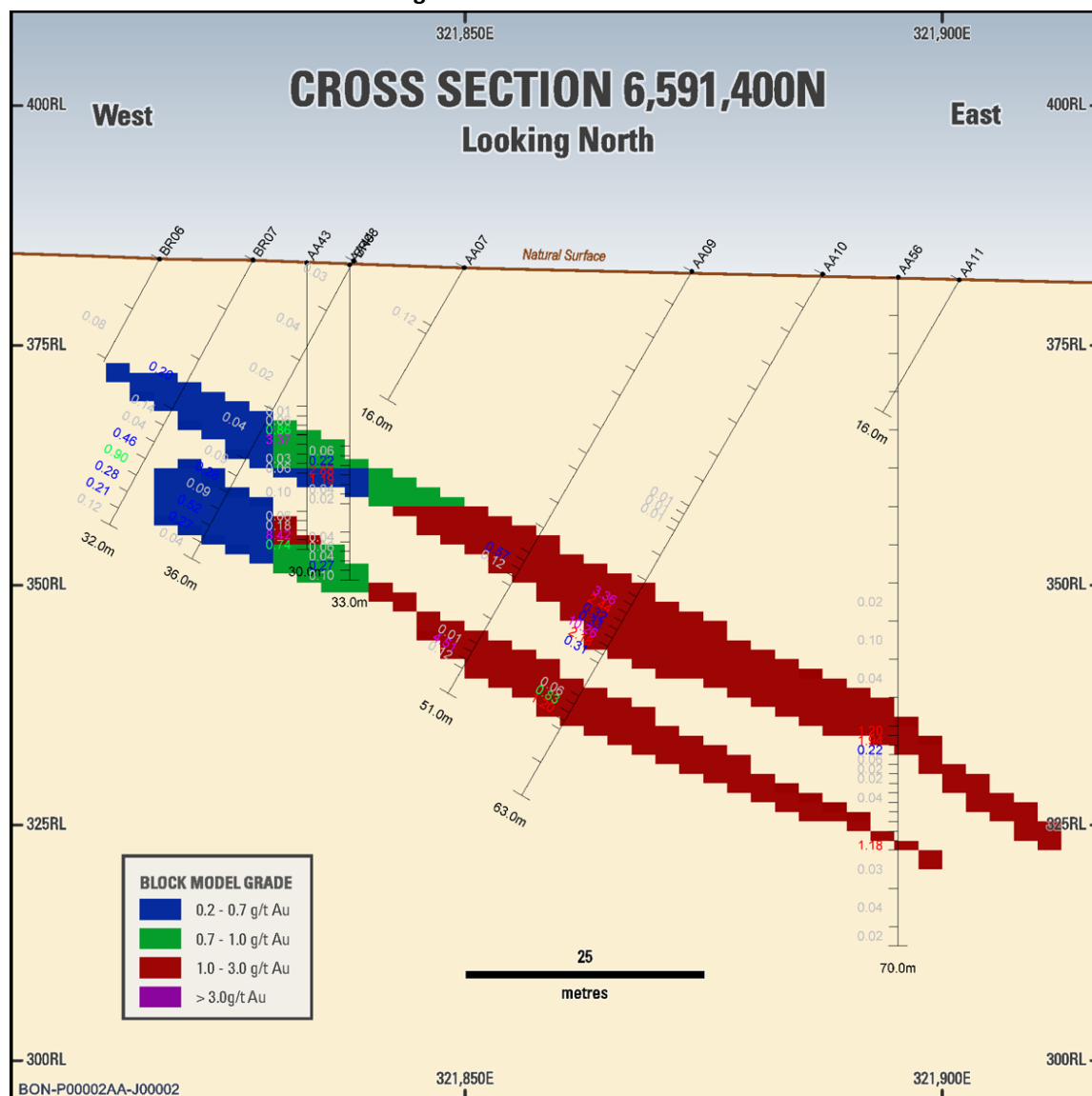
Figure 5. Cross Section 6591400N
