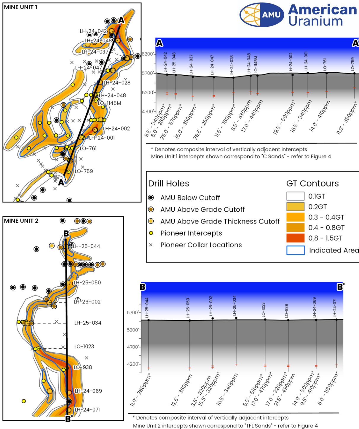
FIGURE 3: CROSS SECTIONS OF MINERALISED DRILL HOLE INTERCEPTS IN THE C SAND HORIZON AND THE TFL SAND HORIZON
