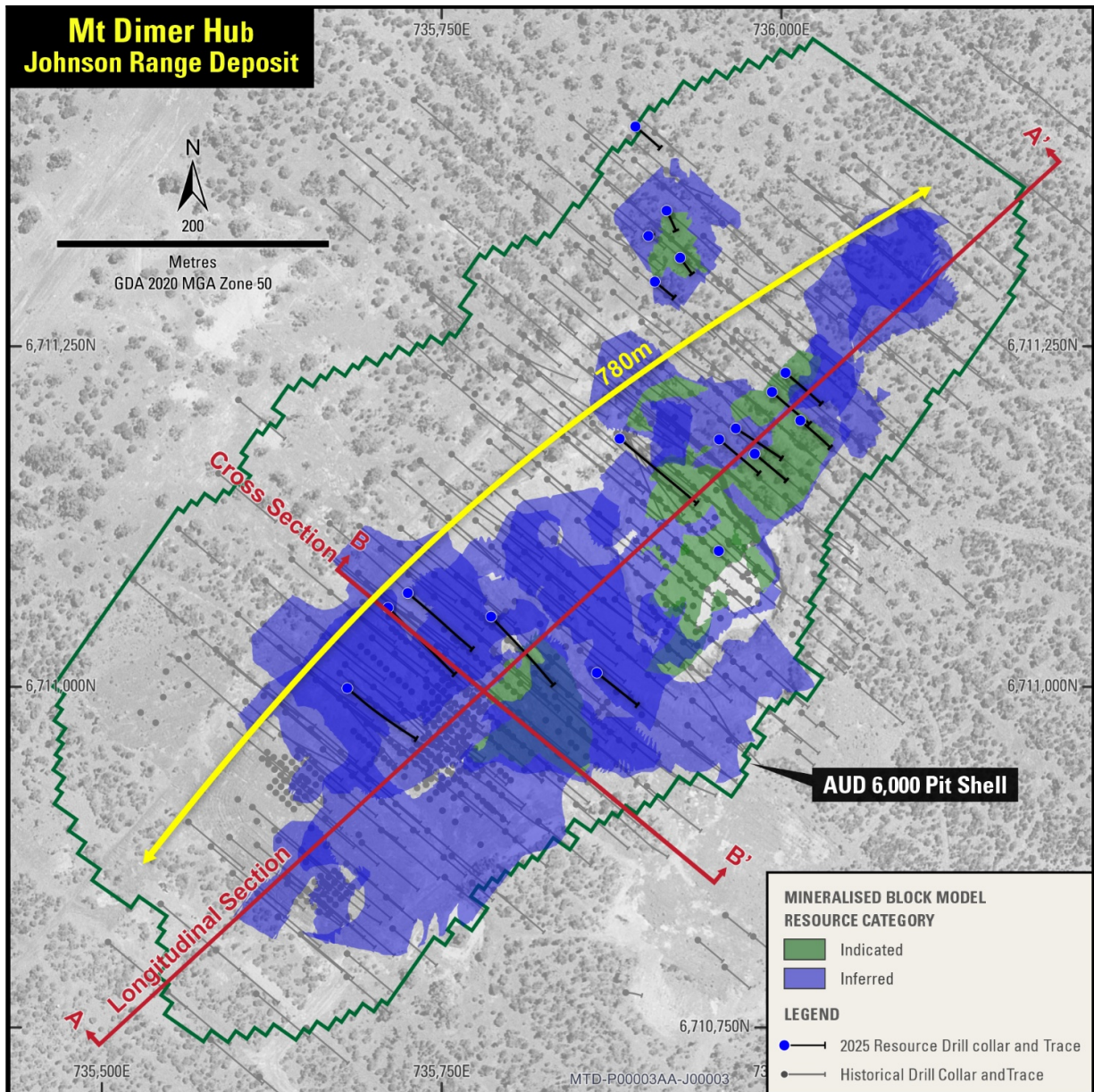
Figure 3 Johnson Range Deposit - MRE
