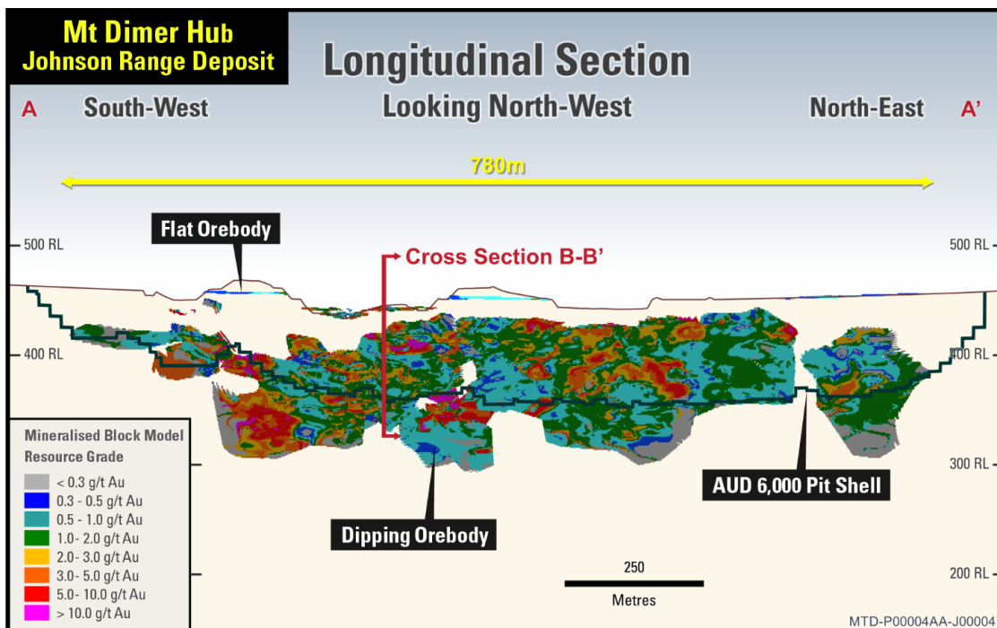
Figure 5 Johnson Range Deposit – Long section
