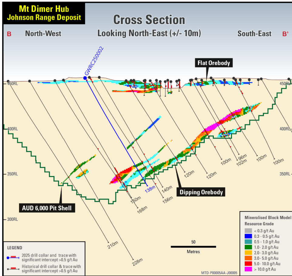
Figure 4 Johnson Range Deposit – Cross section
