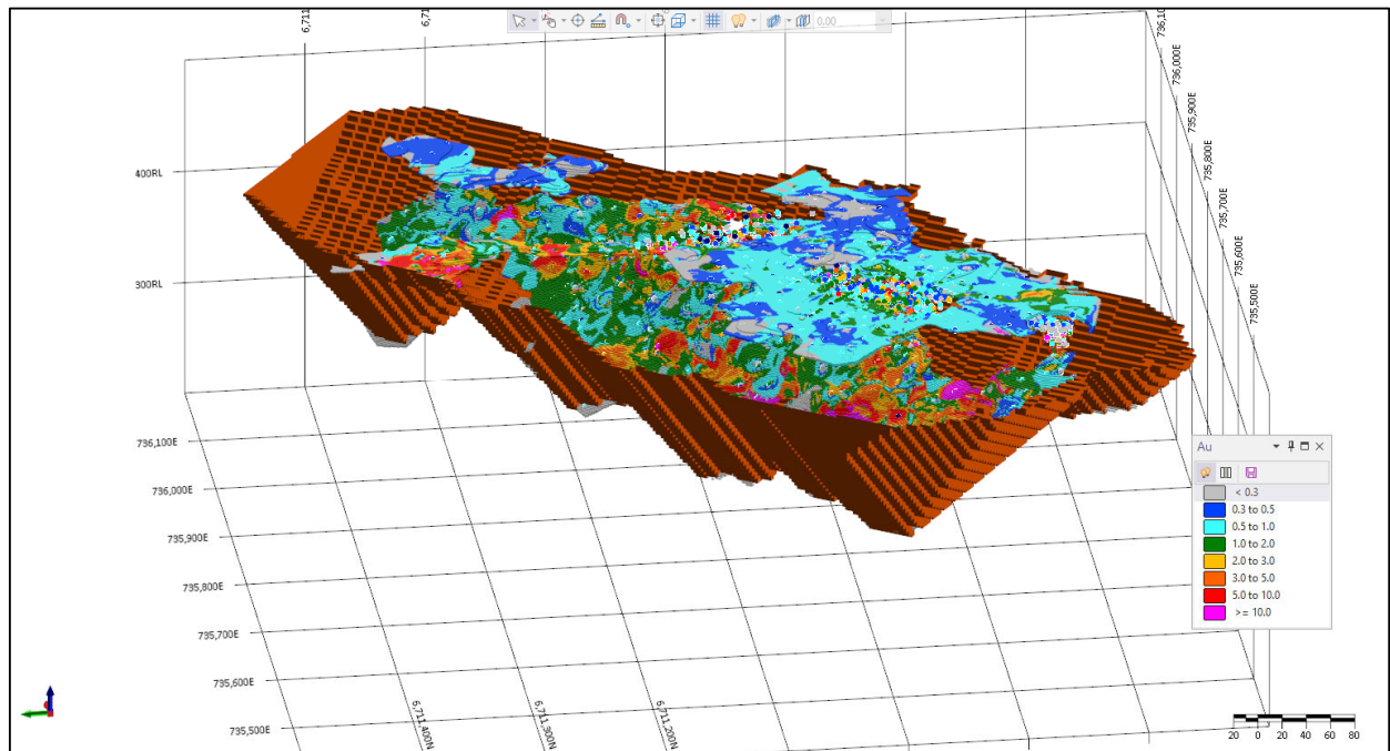
Figure 9 $A6,000 Optimal Pit Shell and Mineralised Block Model
