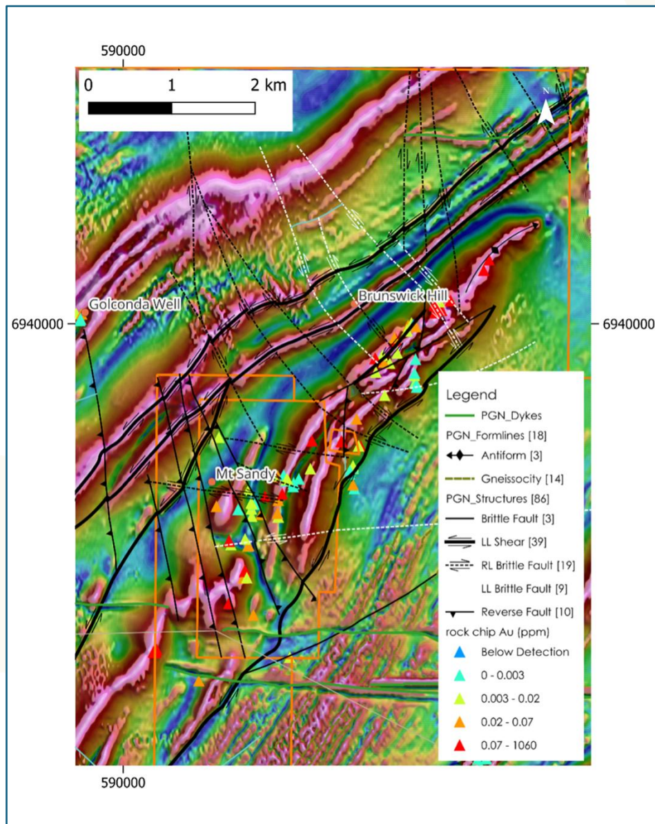
Figure 1: Interpreted structural framework from aeromagnetics and ground gravity with anomalous rock-chip locations highlighting potential structural controls on mineralisation. Background: composite reduced-to-pole (RTP) magnetics (colour) blended with tilt-derivative RTP (grey).
