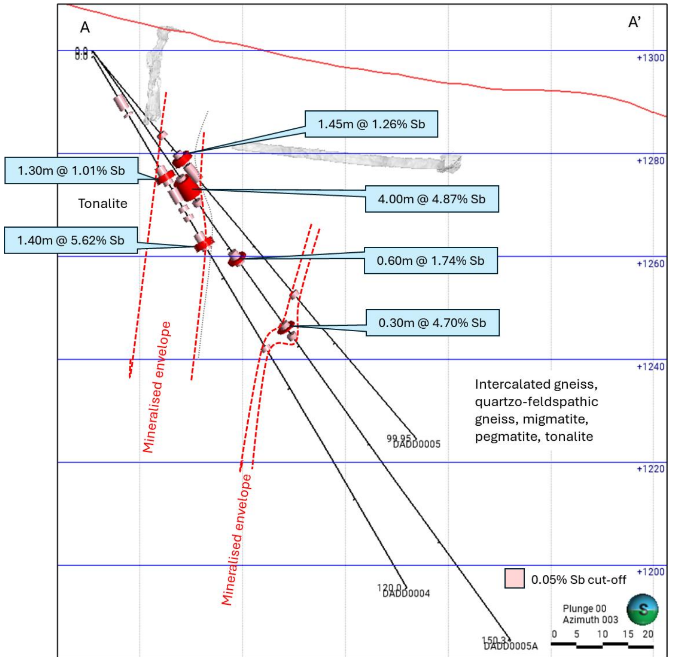
Figure 2: Cross section view of completed diamond drilling on section line A-A' in Figure 1.
