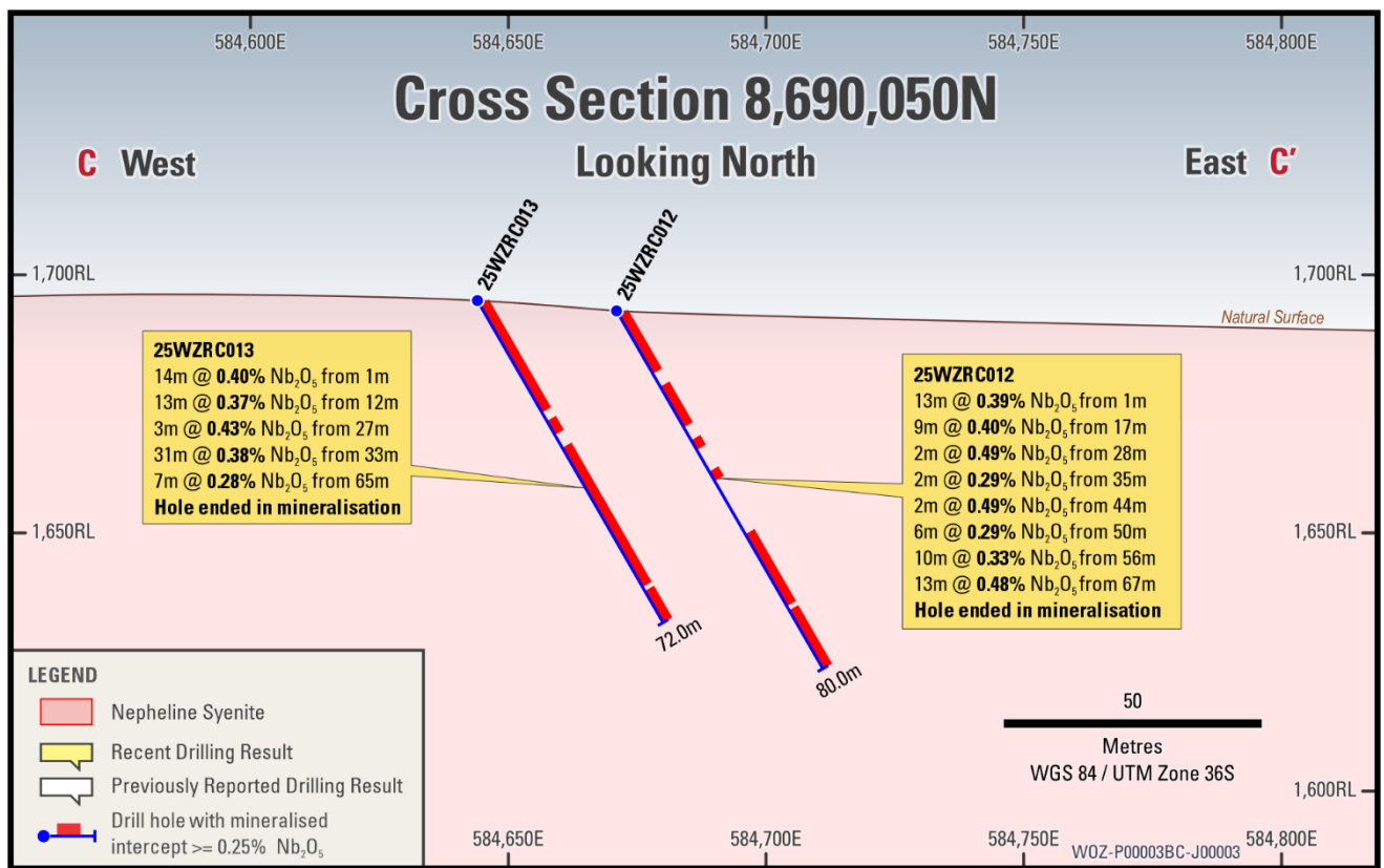
Figure 4: Cross-section 8,690,050 N
