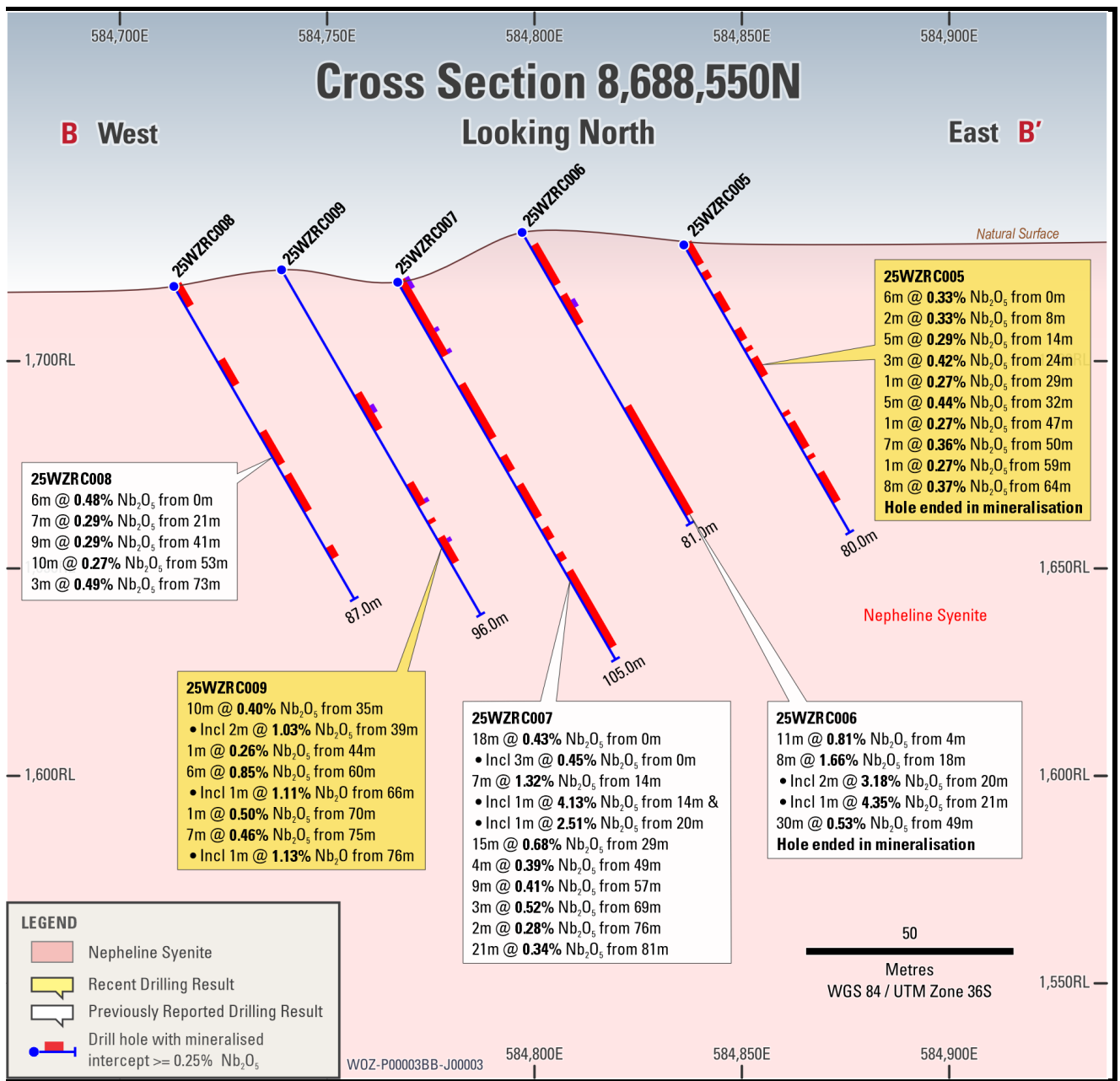
Figure 5: Cross-section 8,688,550 N
