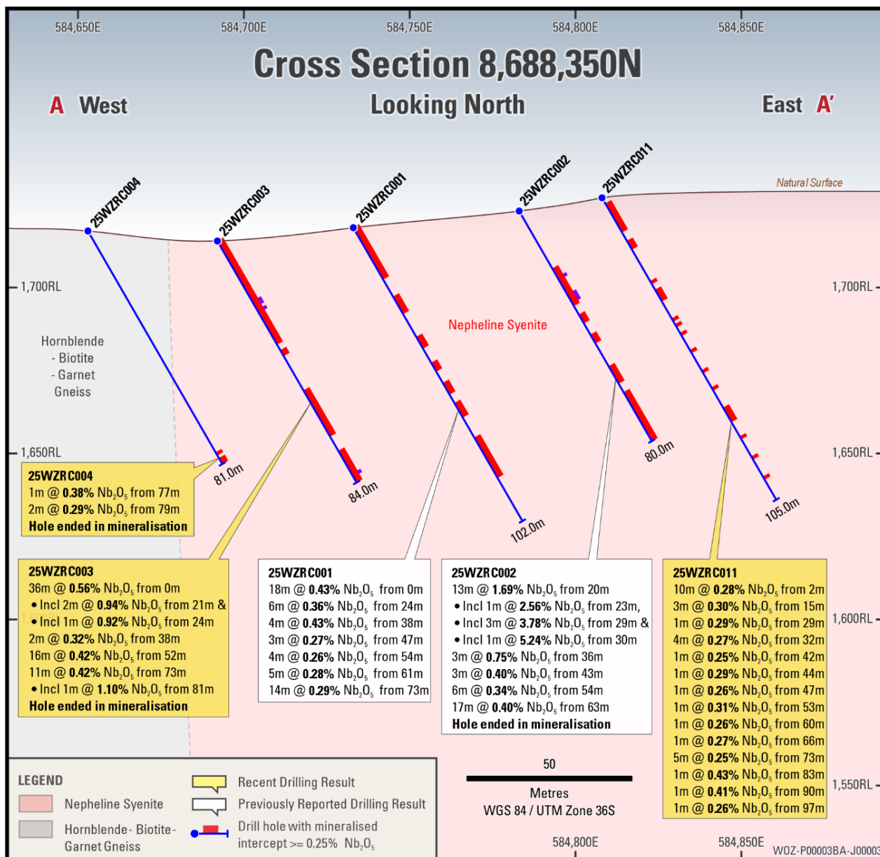
Figure 6: Cross-section 8,688,350 N
