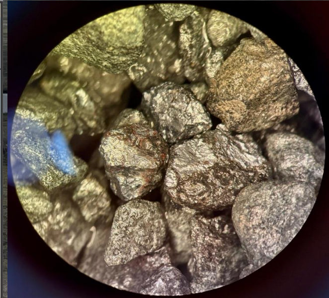
Chalcopyrite rich chips from DAN25005
