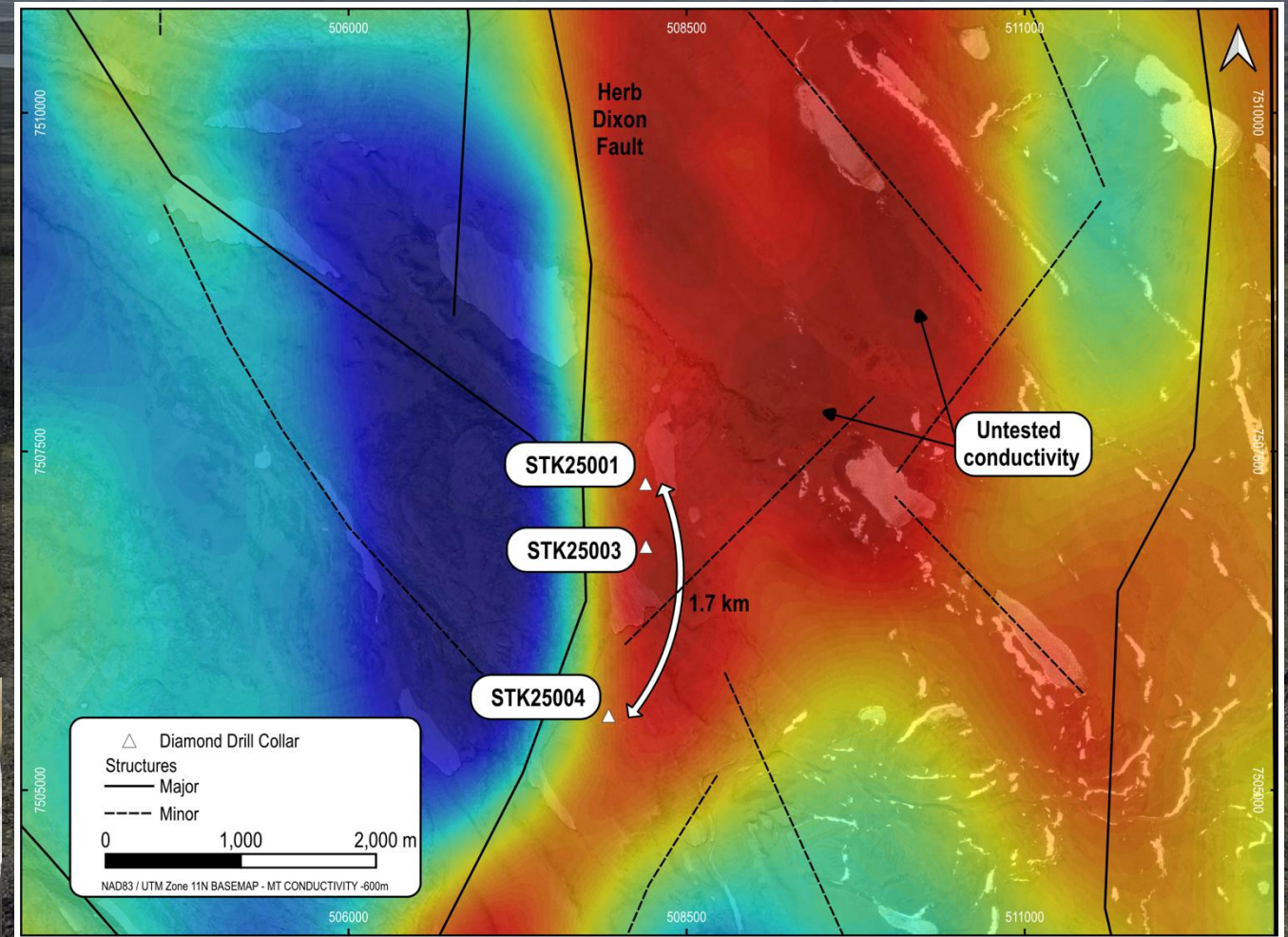
Plan view of 2025 drillholes STK25001, STK25003 & STK25004 into the Stark target. Basemap of conductivity from 2024 MT survey illustrating an untested zone of deep conductivity to the east /northeast of drillholes
